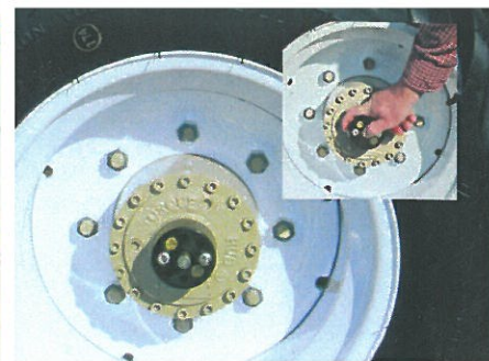
Push Button Free Wheeling Hub for towing or manual positioning.
